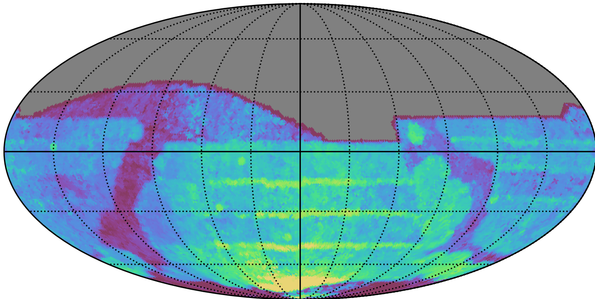
weather_cloudso2v3.4_10yrs All sky all bands: Median Season Length
