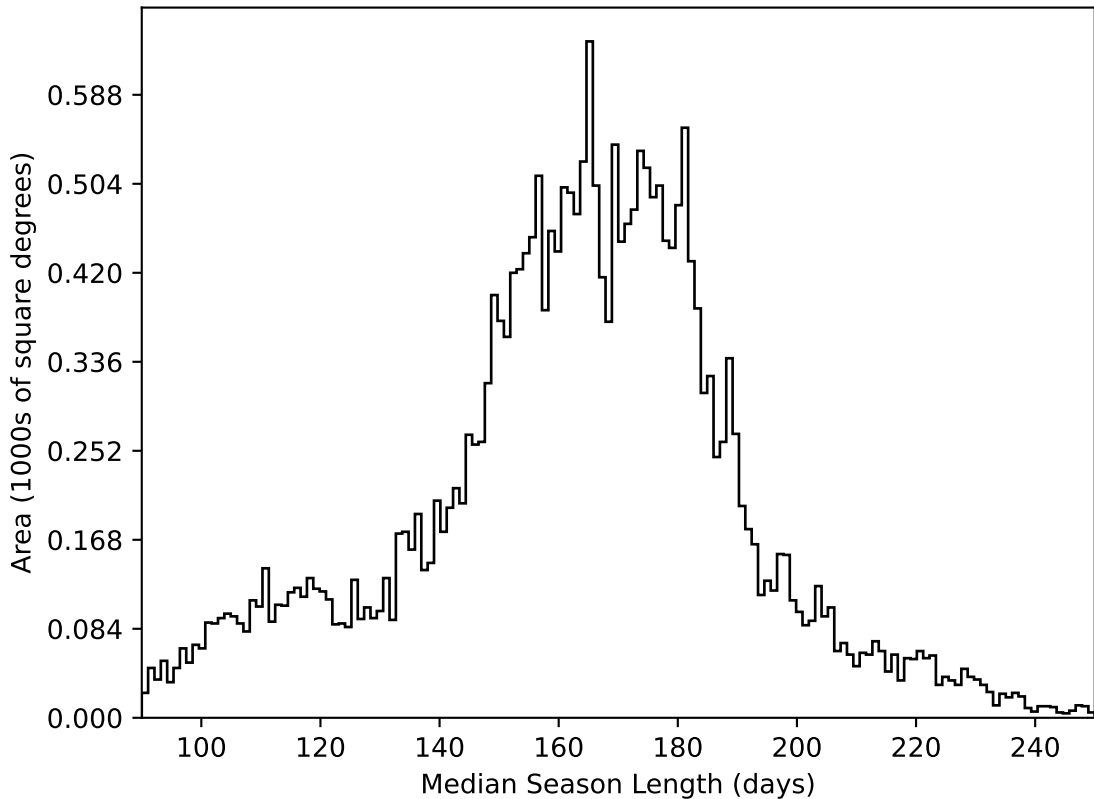
weather_cloudso2v3.4_10yrs All sky all bands: Median Season Length
