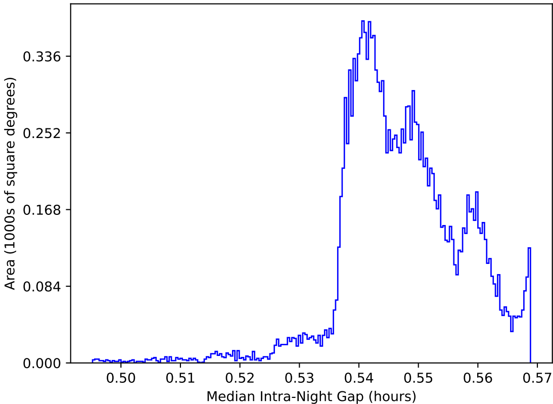
weather_cloudso2v3.4_10yrs WFD: Median Intra-Night Gap
