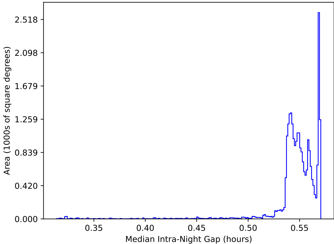
weather_cloudso2v3.4_10yrs All sky: Median Intra-Night Gap
