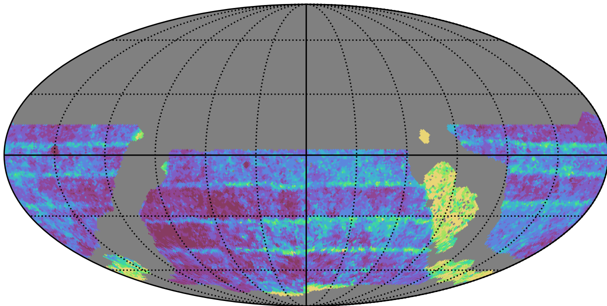
weather_cloudso2v3.4_10yrs WFD z band: Median Inter-Night Gap
