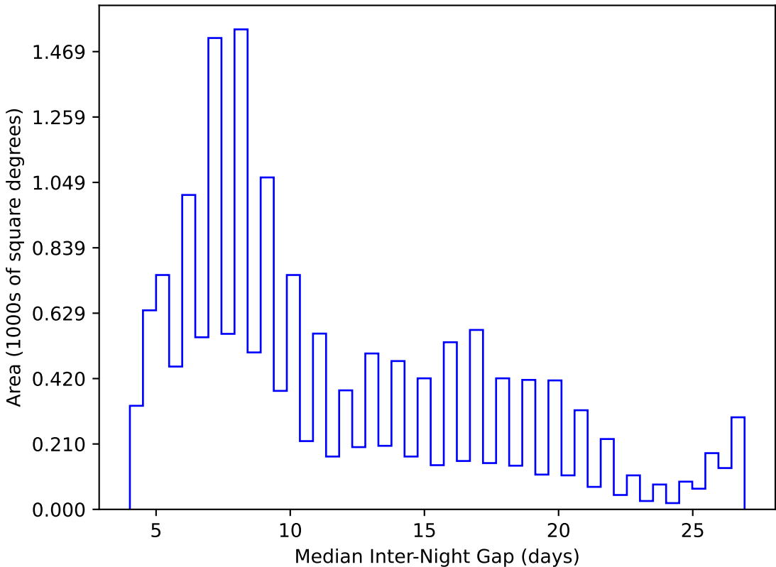
weather_cloudso2v3.4_10yrs WFD y band: Median Inter-Night Gap
