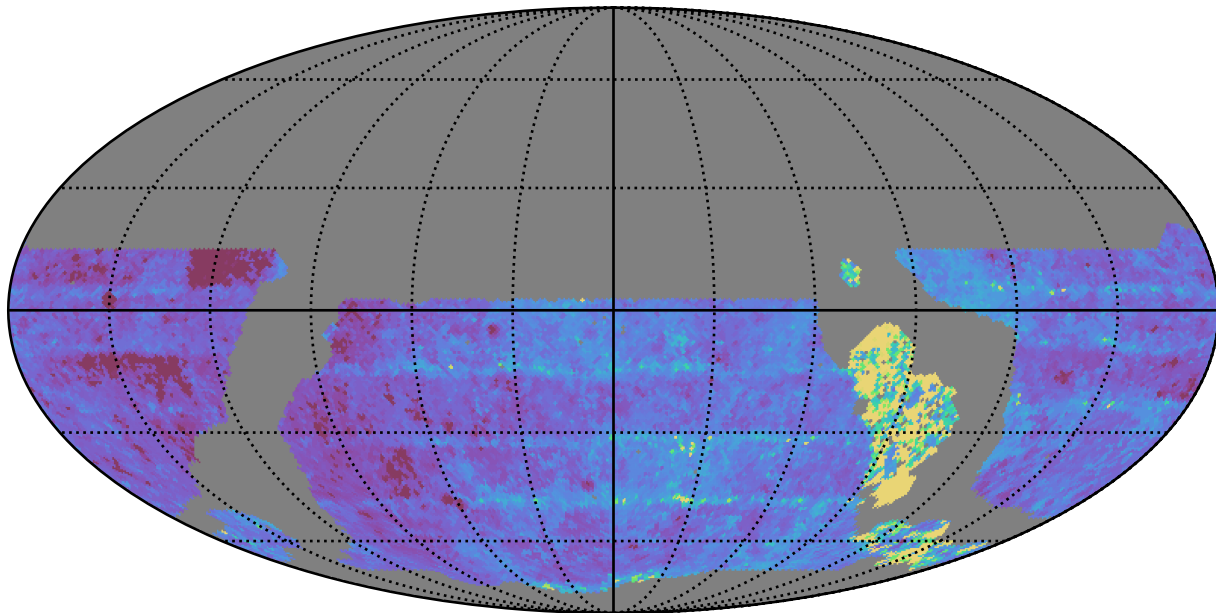
weather_cloudso2v3.4_10yrs WFD u band: Median Inter-Night Gap
