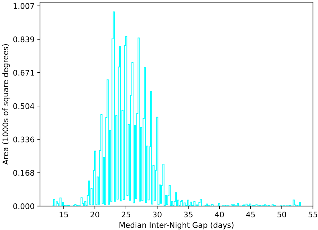
weather_cloudso2v3.4_10yrs WFD u band: Median Inter-Night Gap
