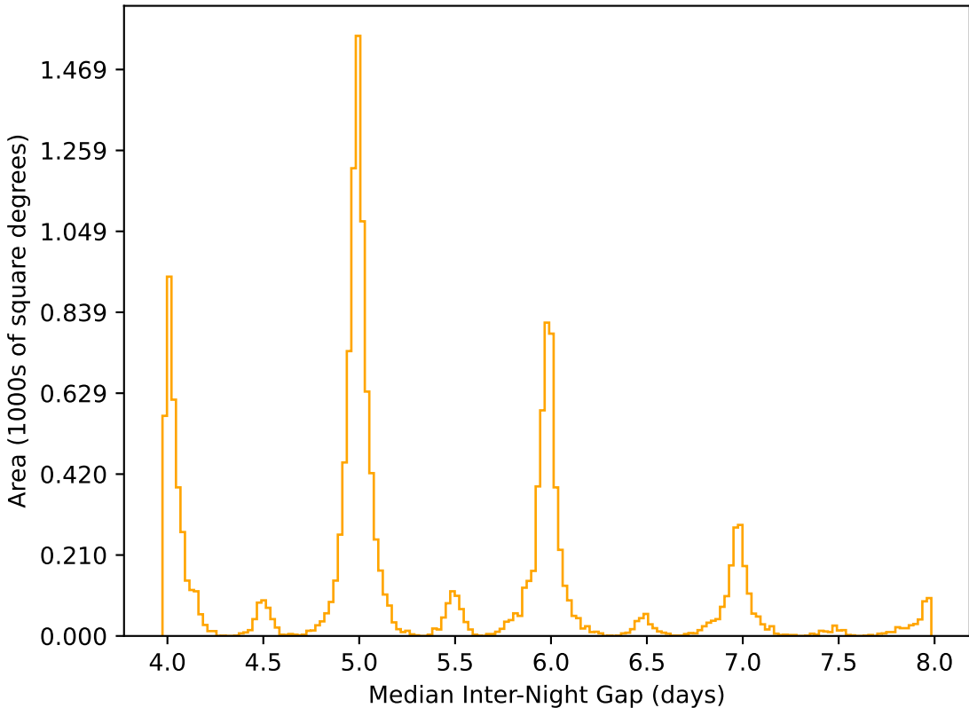
weather_cloudso2v3.4_10yrs WFD r band: Median Inter-Night Gap
