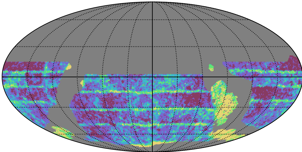
weather_cloudso2v3.4_10yrs WFD i band: Median Inter-Night Gap
