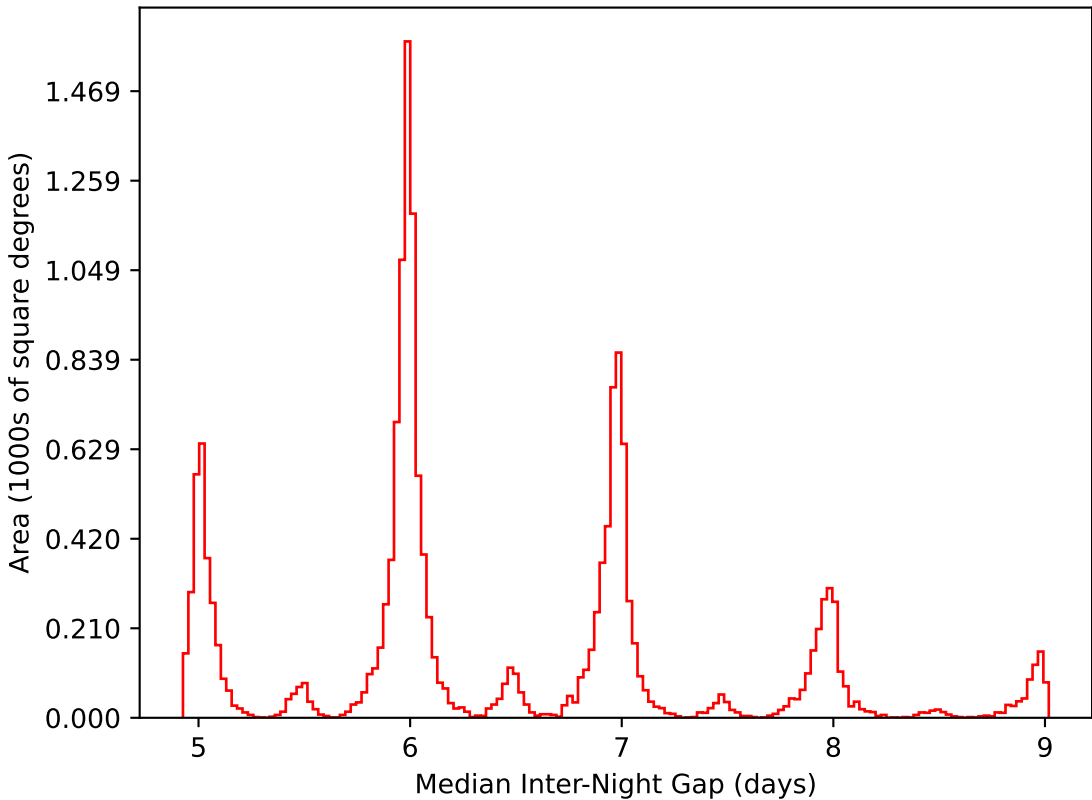
weather_cloudso2v3.4_10yrs WFD i band: Median Inter-Night Gap
