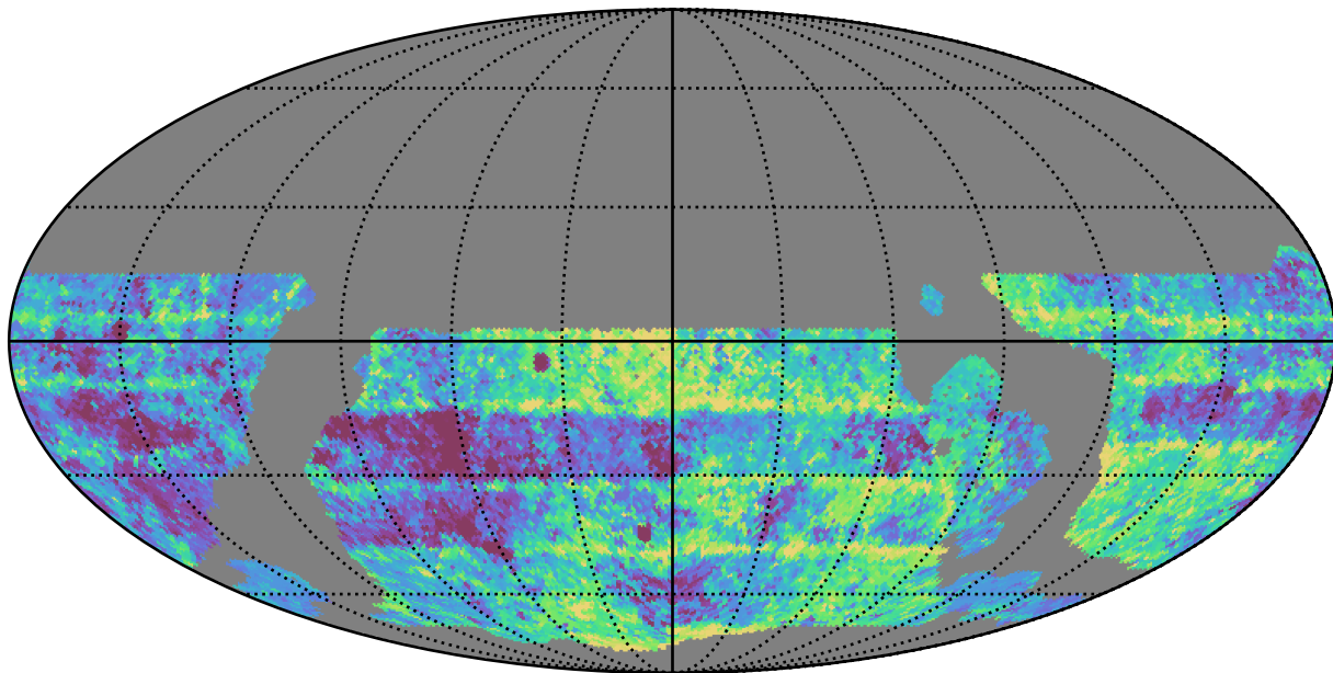
weather_cloudso2v3.4_10yrs WFD g band: Median Inter-Night Gap
