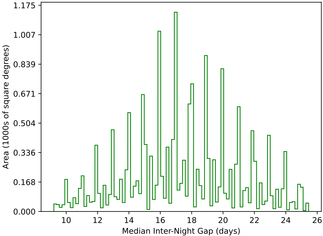
weather_cloudso2v3.4_10yrs WFD g band: Median Inter-Night Gap
