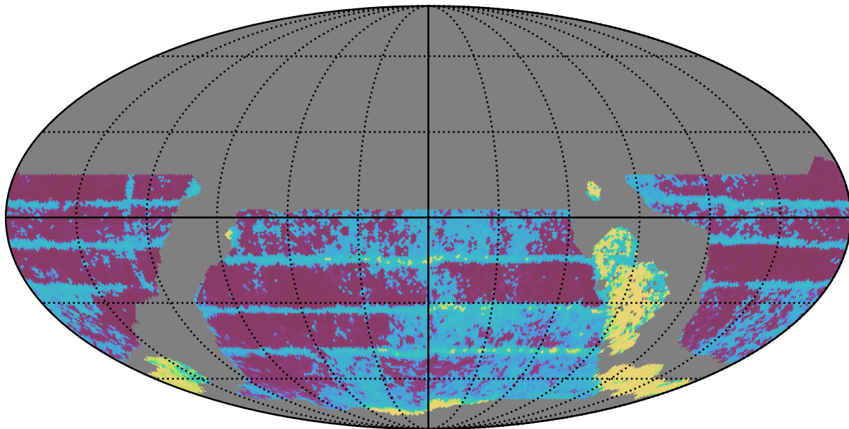
weather_cloudso2v3.4_10yrs WFD all bands: Median Inter-Night Gap
