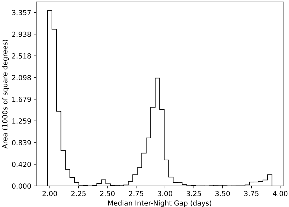
weather_cloudso2v3.4_10yrs WFD all bands: Median Inter-Night Gap
