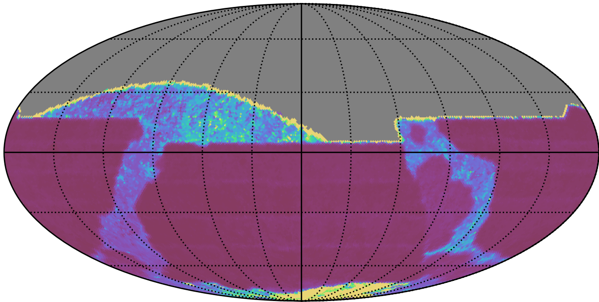
weather_cloudso2v3.4_10yrs All sky z band: Median Inter-Night Gap
