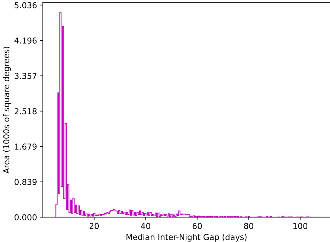
weather_cloudso2v3.4_10yrs All sky z band: Median Inter-Night Gap
