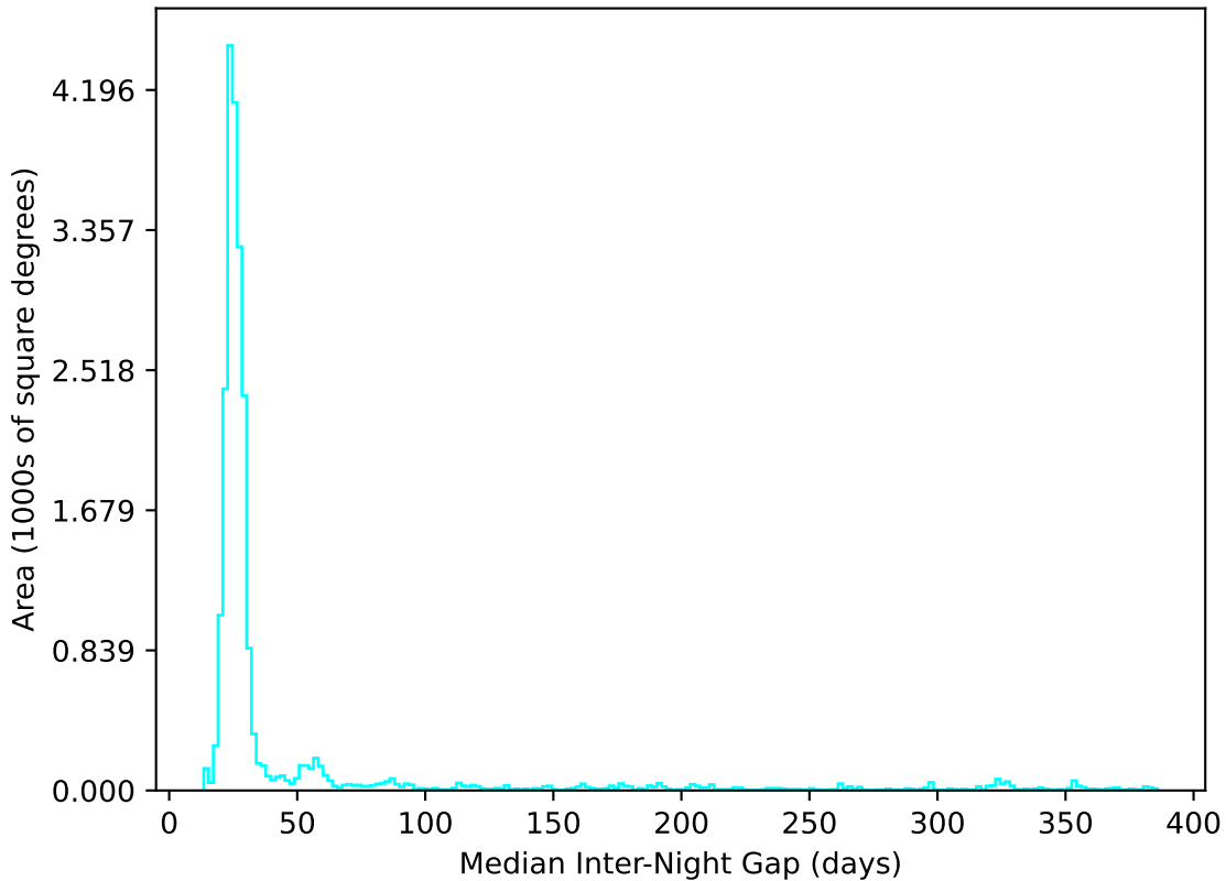
weather_cloudso2v3.4_10yrs All sky u band: Median Inter-Night Gap
