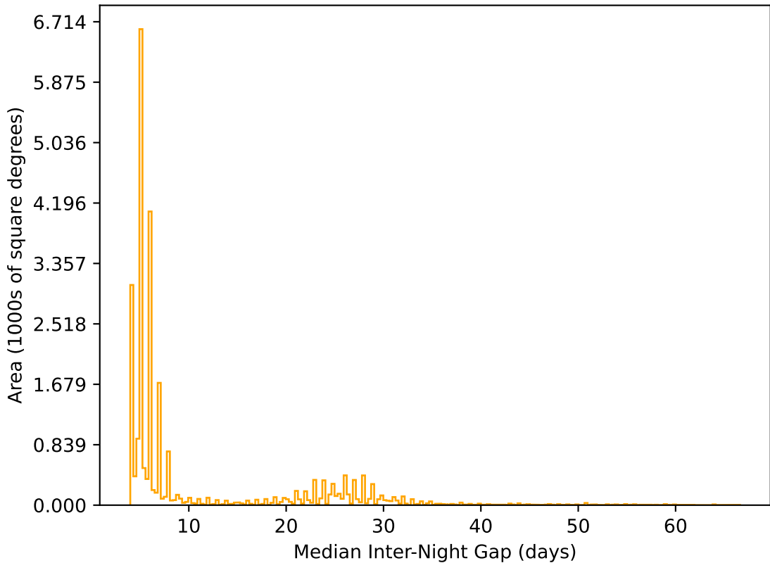
weather_cloudso2v3.4_10yrs All sky r band: Median Inter-Night Gap
