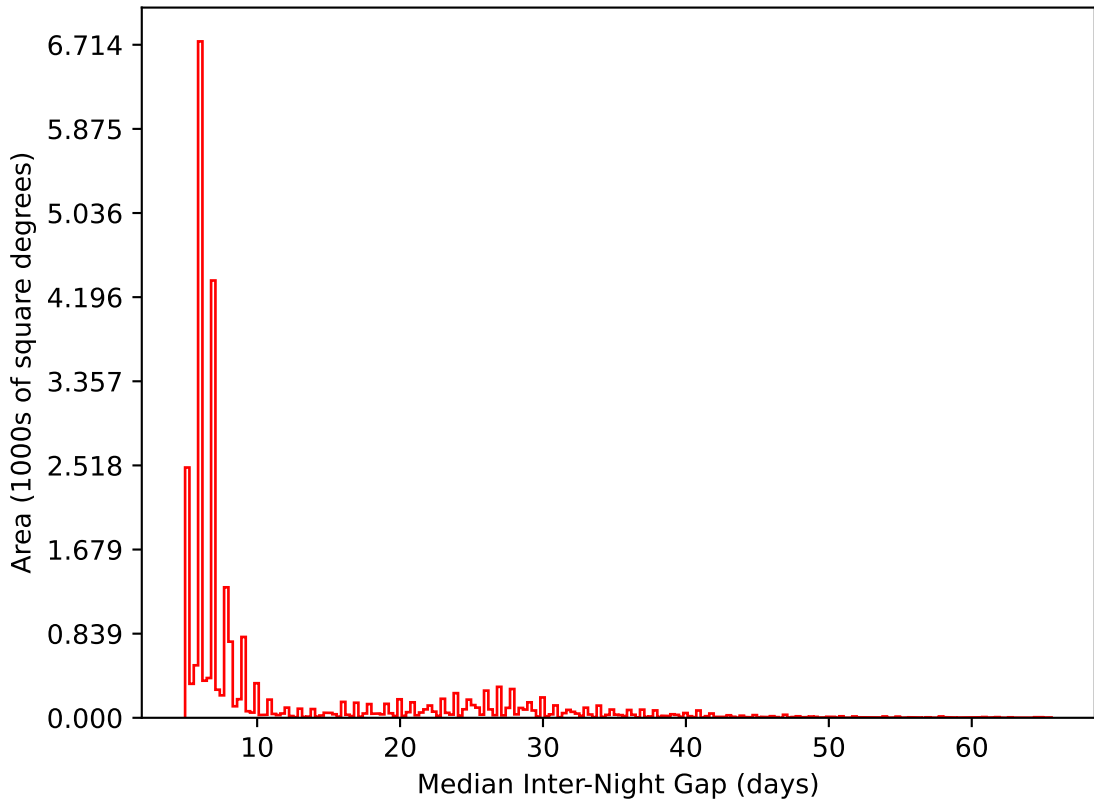
weather_cloudso2v3.4_10yrs All sky i band: Median Inter-Night Gap
