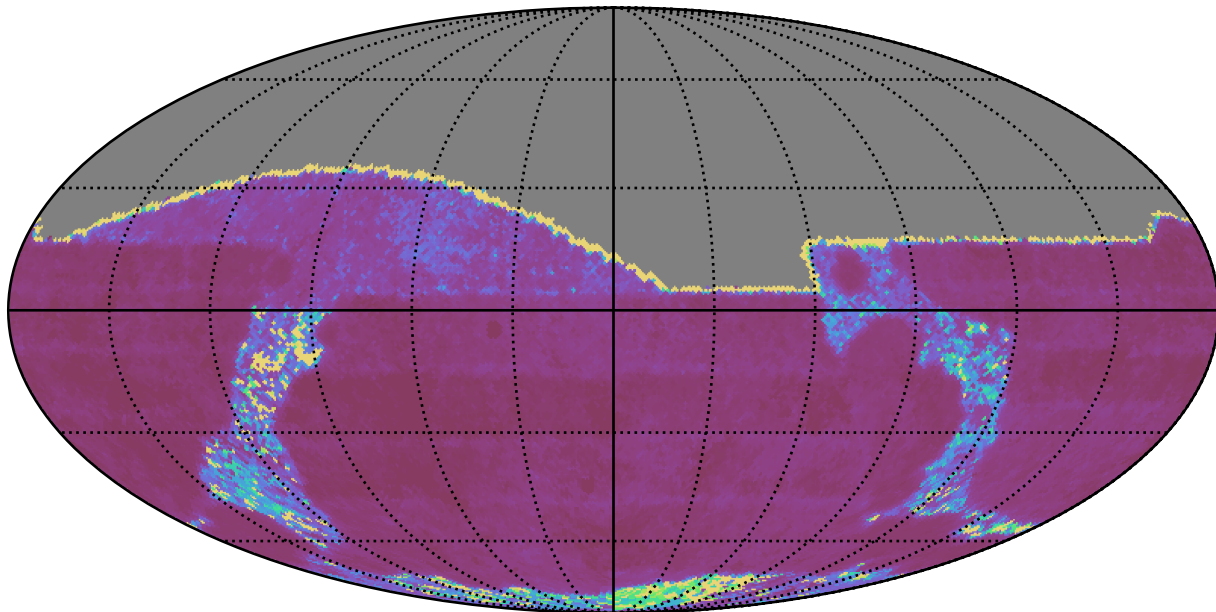
weather_cloudso2v3.4_10yrs All sky g band: Median Inter-Night Gap
