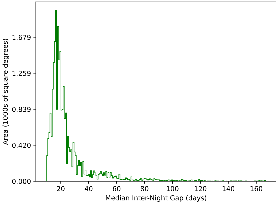
weather_cloudso2v3.4_10yrs All sky g band: Median Inter-Night Gap
