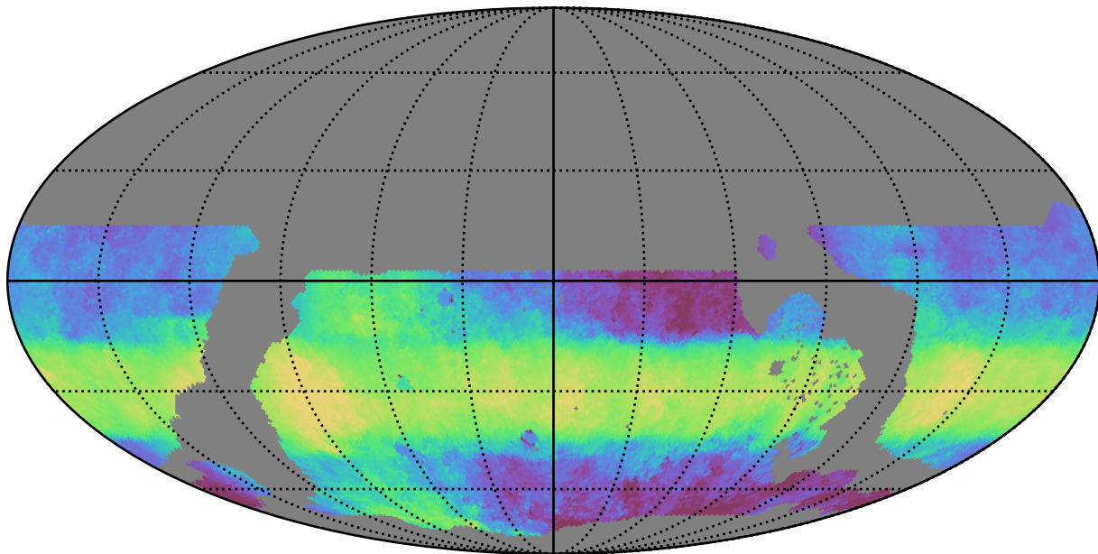
weather_cloudso2v3.4_10yrs WFD z band: Median HA
