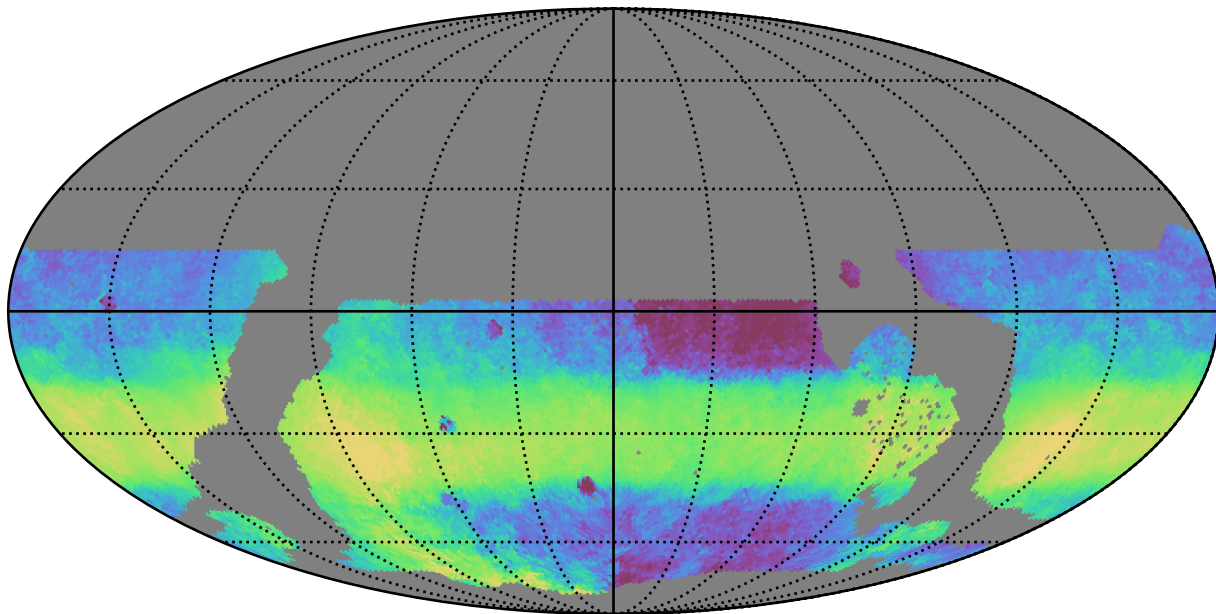
weather_cloudso2v3.4_10yrs WFD y band: Median HA
