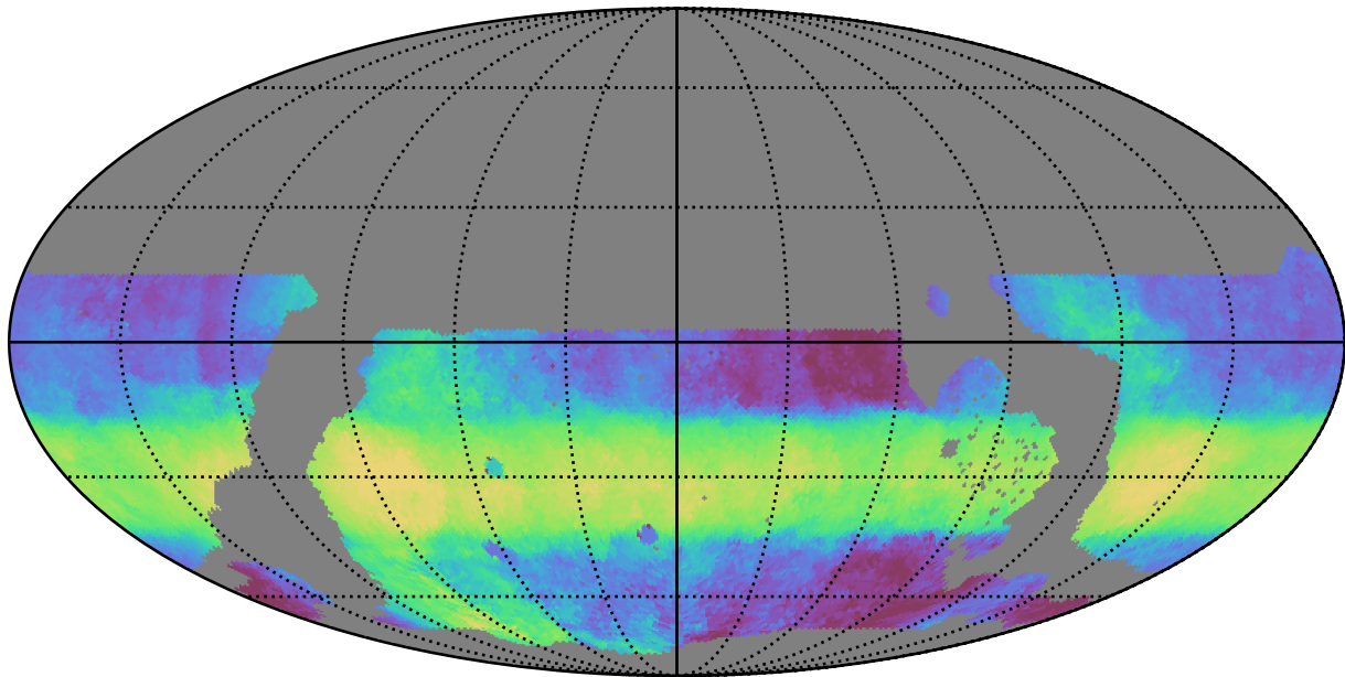
weather_cloudso2v3.4_10yrs WFD r band: Median HA
