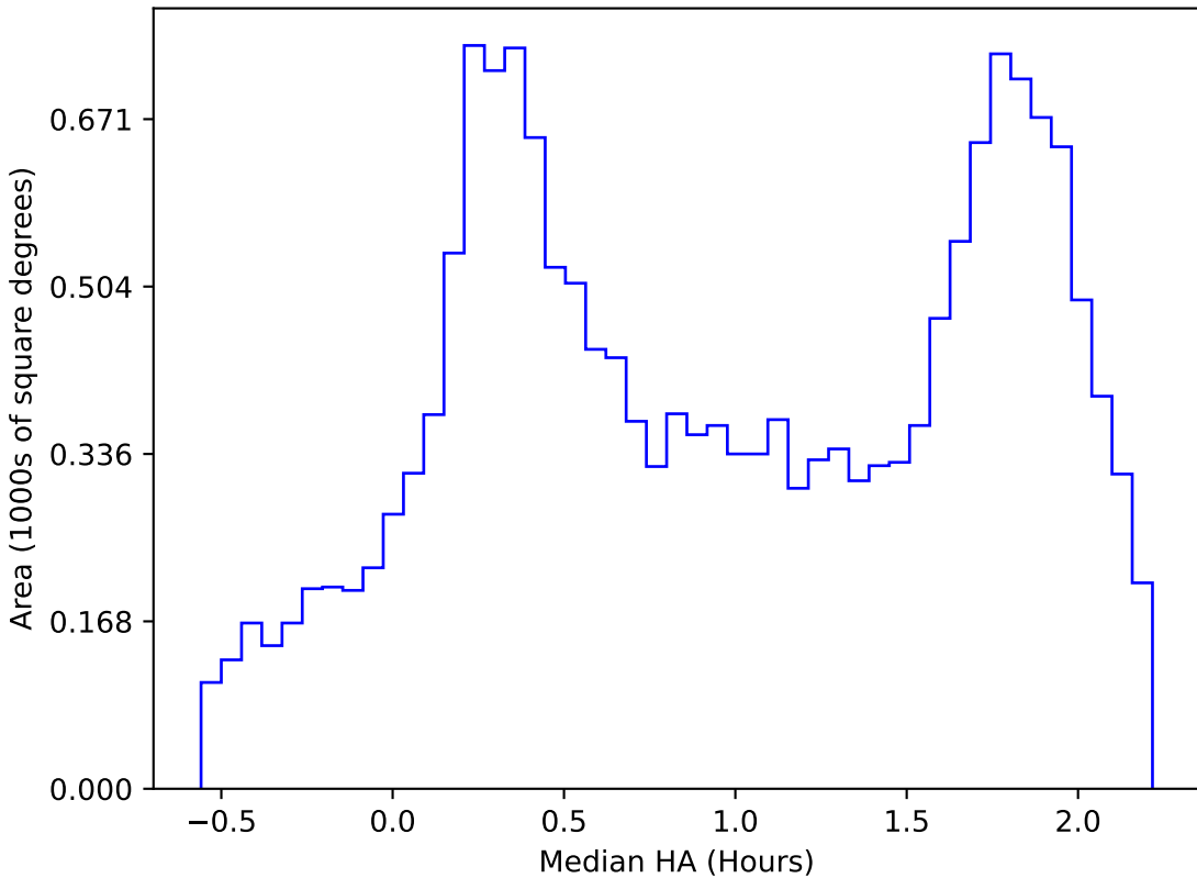
weather_cloudso2v3.4_10yrs WFD r band: Median HA
