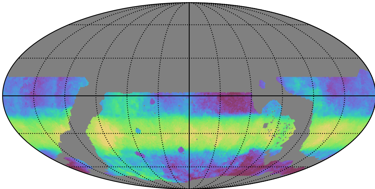
weather_cloudso2v3.4_10yrs WFD i band: Median HA
