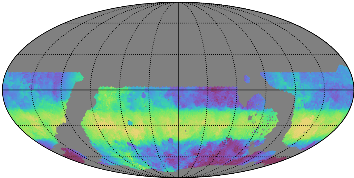
weather_cloudso2v3.4_10yrs WFD g band: Median HA
