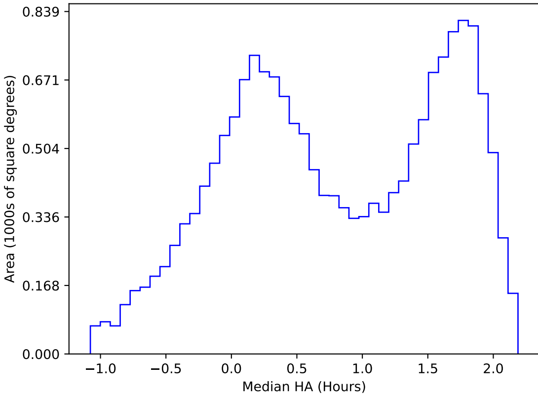
weather_cloudso2v3.4_10yrs WFD g band: Median HA
