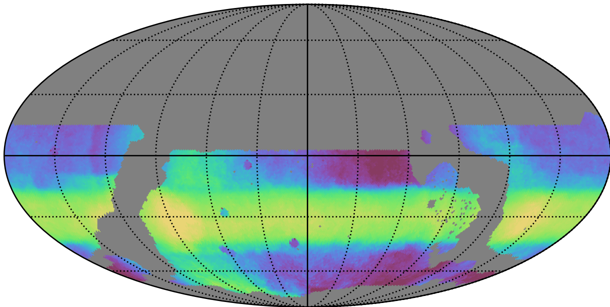
weather_cloudso2v3.4_10yrs WFD all bands: Median HA
