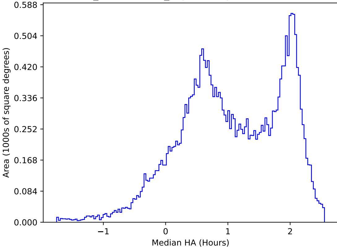
weather_cloudso2v3.4_10yrs All sky z band: Median HA
