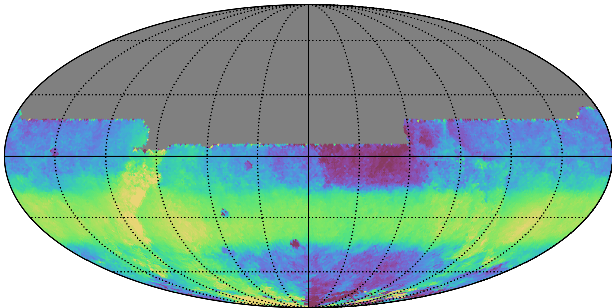
weather_cloudso2v3.4_10yrs All sky y band: Median HA
