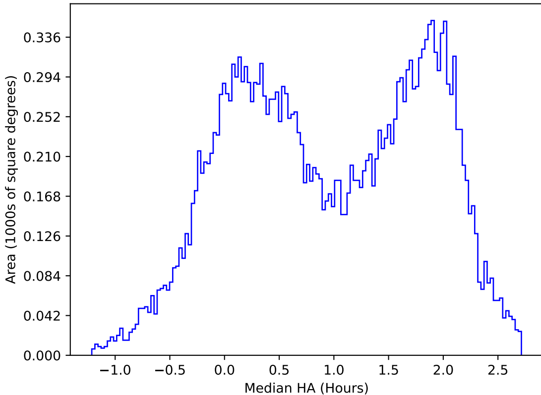
weather_cloudso2v3.4_10yrs All sky u band: Median HA
