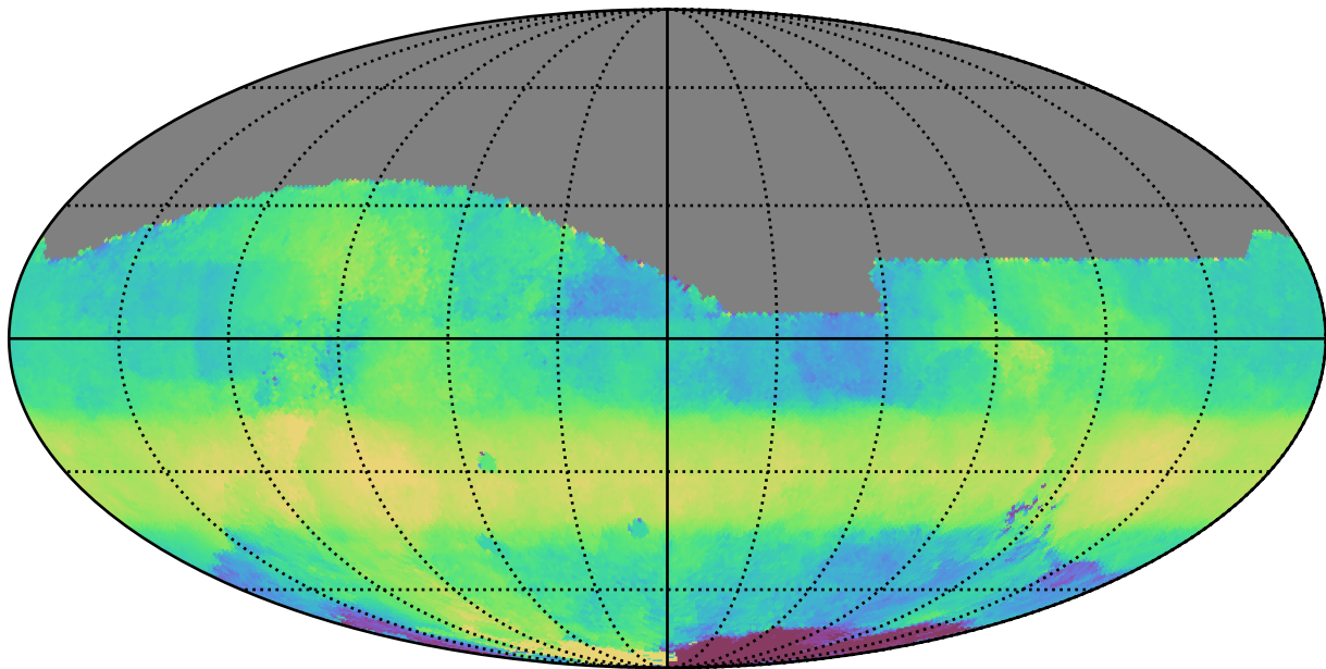
weather_cloudso2v3.4_10yrs All sky r band: Median HA
