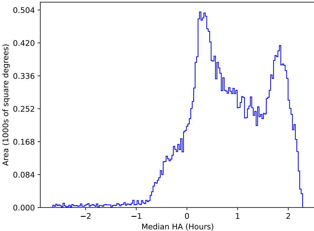
weather_cloudso2v3.4_10yrs All sky r band: Median HA
