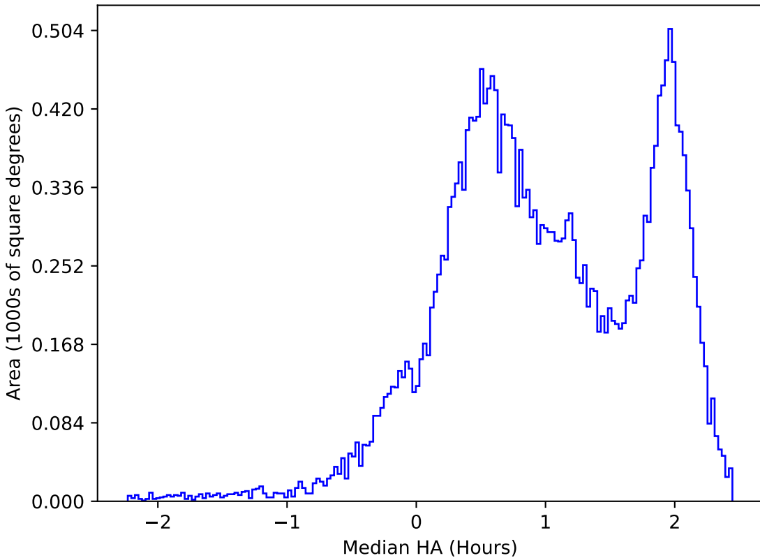
weather_cloudso2v3.4_10yrs All sky i band: Median HA
