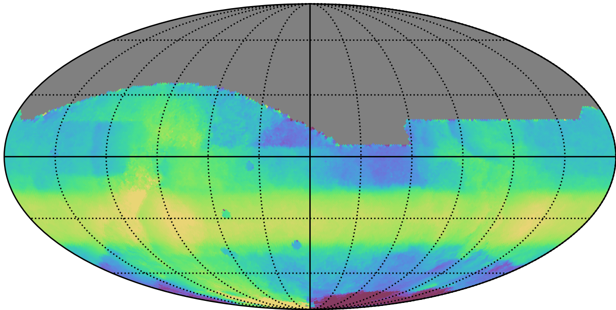
weather_cloudso2v3.4_10yrs All sky all bands: Median HA
