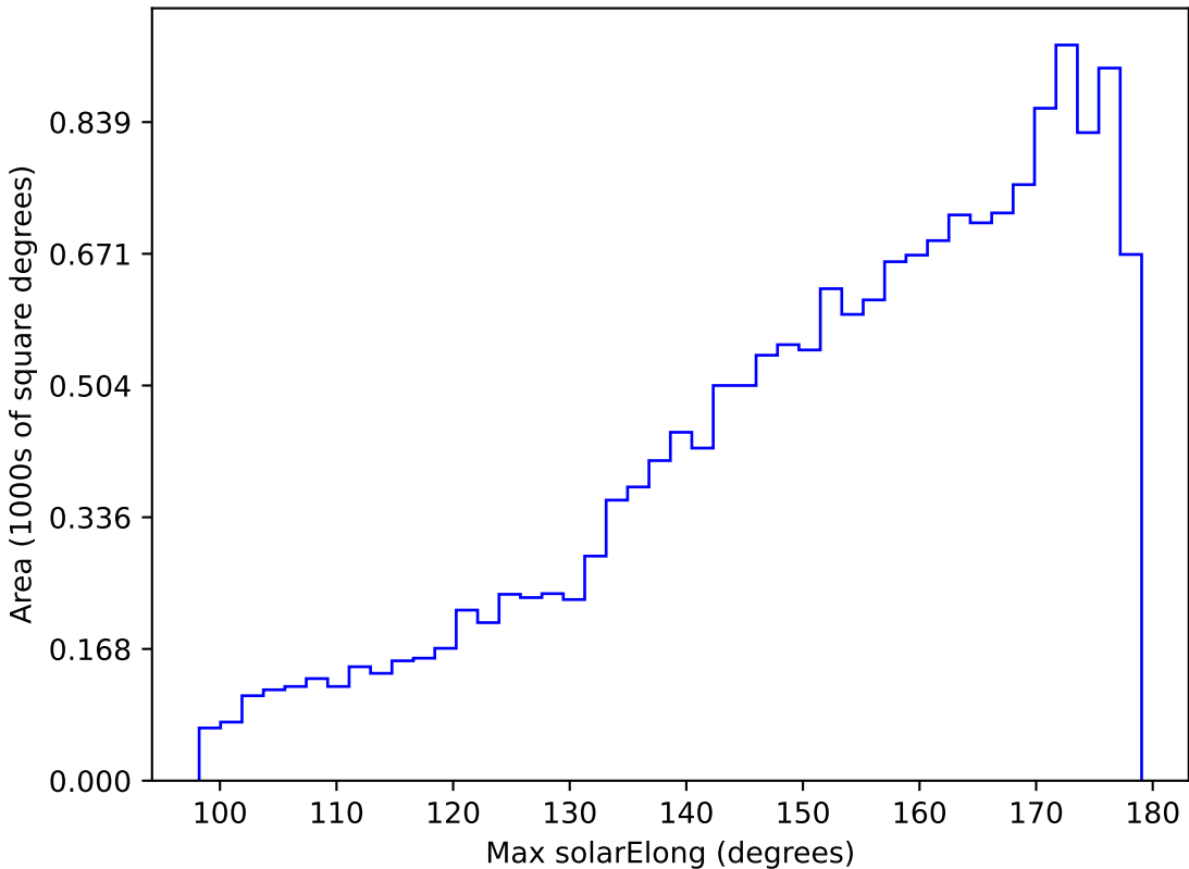
weather_cloudso2v3.4_10yrs WFD u band: Max solarElong
