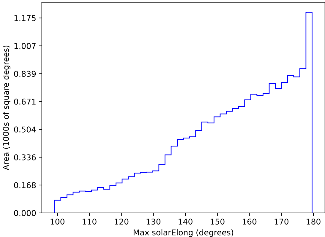
weather_cloudso2v3.4_10yrs WFD all bands: Max solarElong
