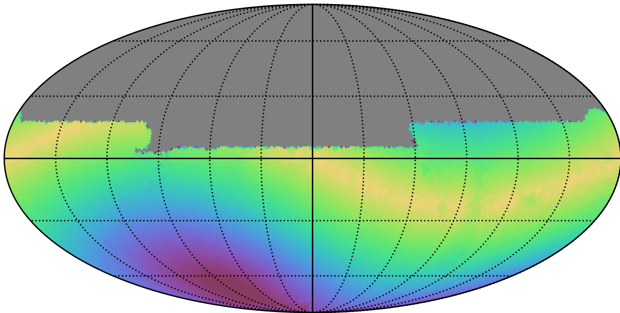
weather_cloudso2v3.4_10yrs All sky u band: Max solarElong
