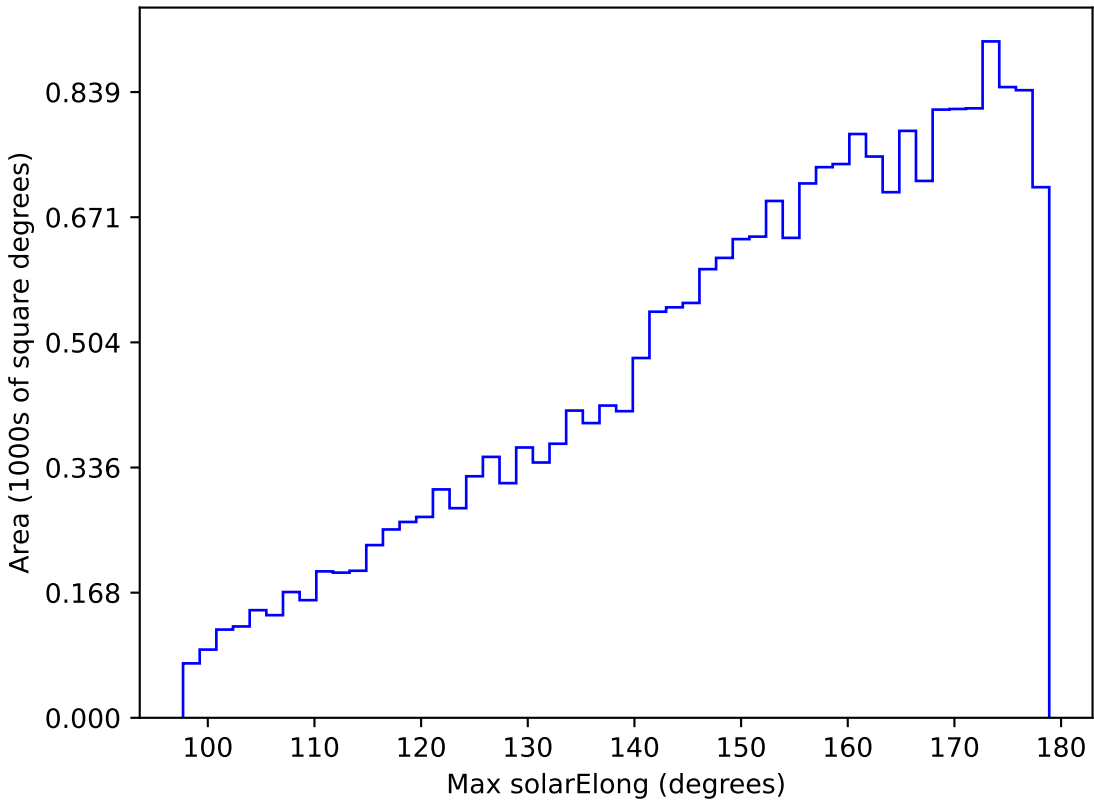
weather_cloudso2v3.4_10yrs All sky u band: Max solarElong
