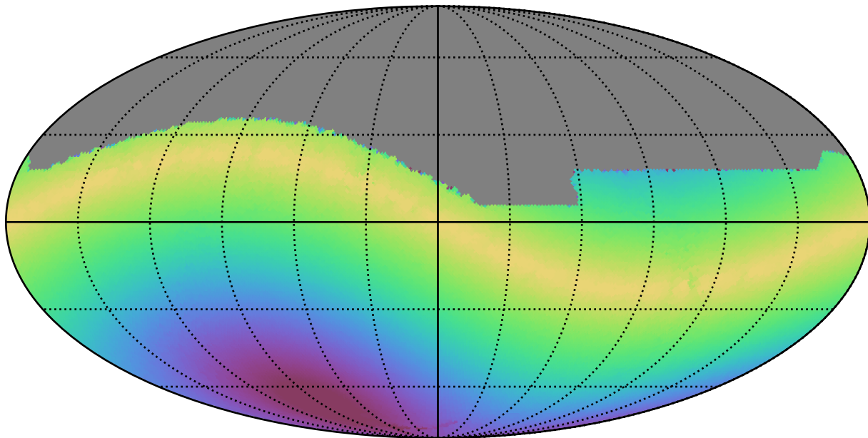
weather_cloudso2v3.4_10yrs All sky r band: Max solarElong
