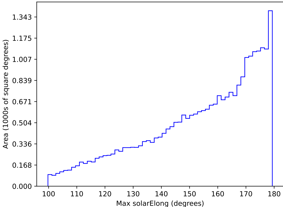
weather_cloudso2v3.4_10yrs All sky r band: Max solarElong
