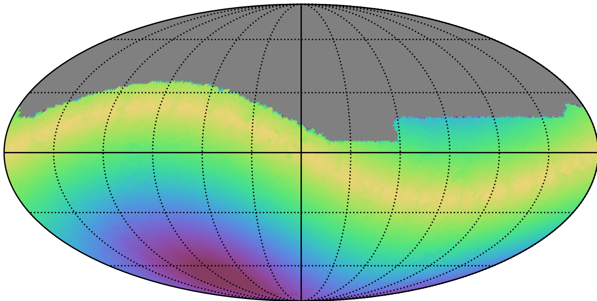
weather_cloudso2v3.4_10yrs All sky g band: Max solarElong
