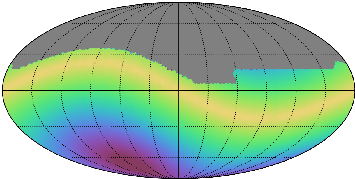
weather_cloudso2v3.4_10yrs All sky all bands: Max solarElong
