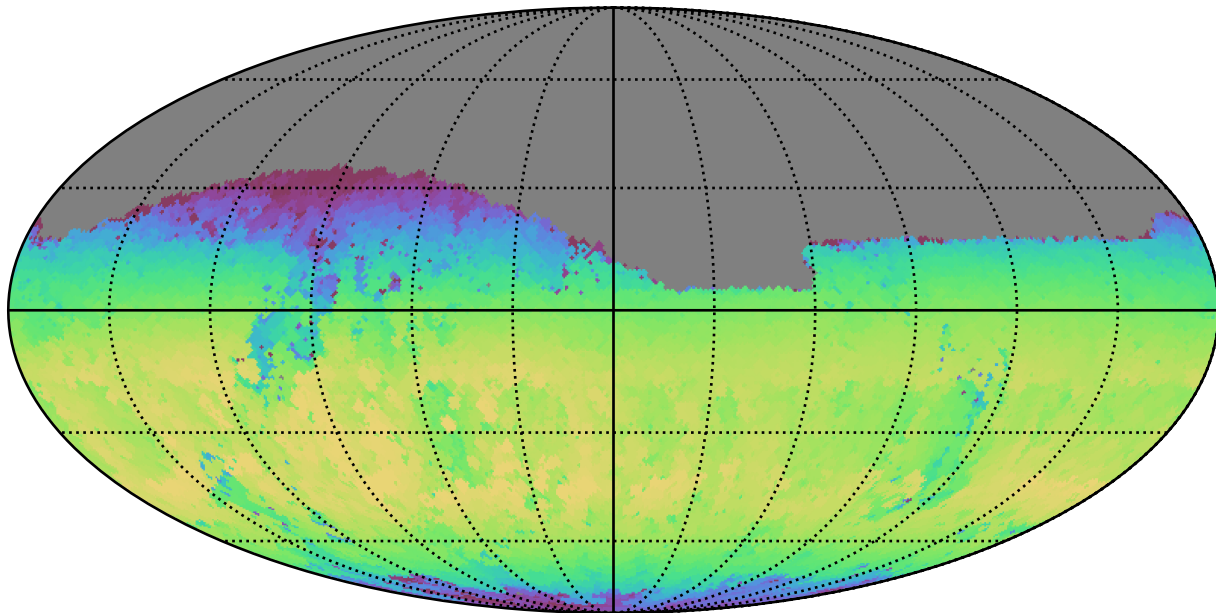
weather_cloudso2v3.4_10yrs Yr 1 z band: Max skyBrightness
