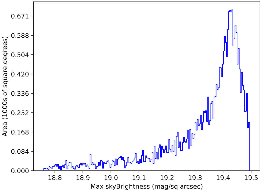
weather_cloudso2v3.4_10yrs Yr 1 z band: Max skyBrightness
