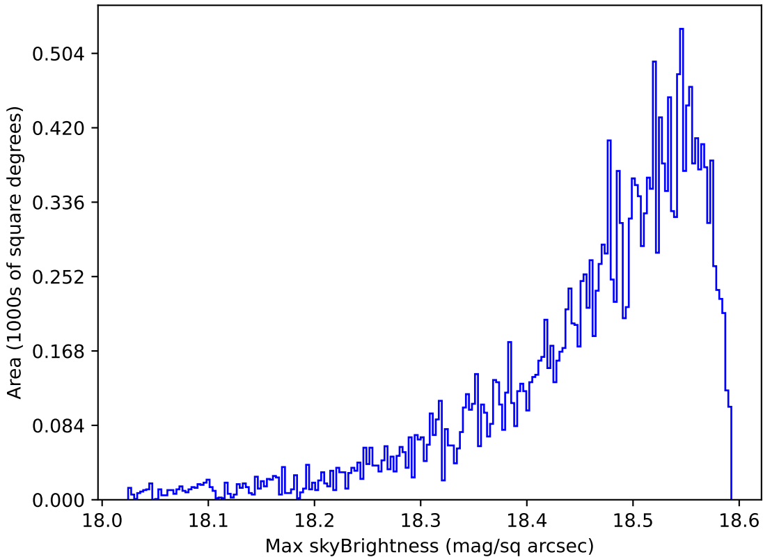
weather_cloudso2v3.4_10yrs Yr 1 y band: Max skyBrightness
