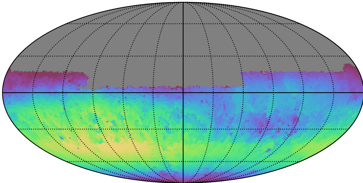
weather_cloudso2v3.4_10yrs Yr 1 u band: Max skyBrightness
