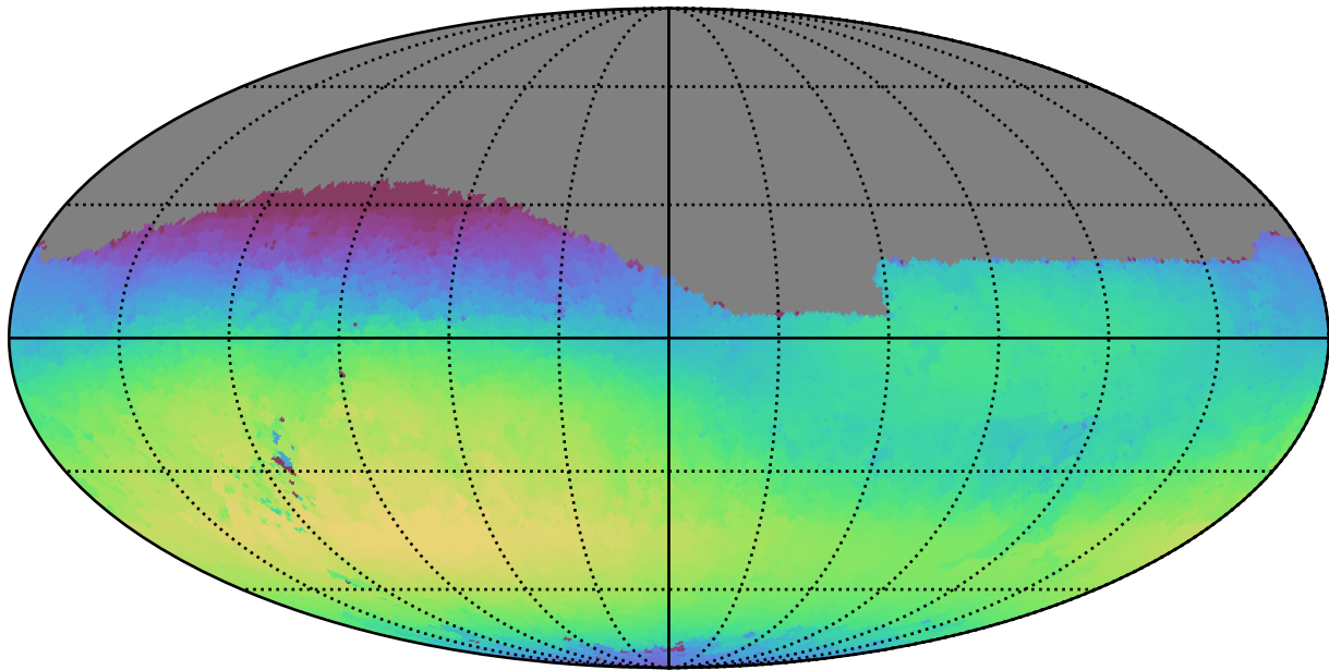
weather_cloudso2v3.4_10yrs Yr 1 r band: Max skyBrightness
